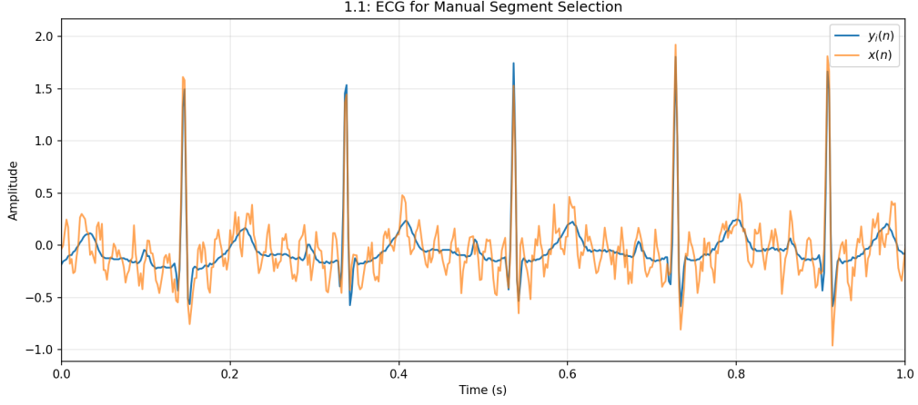
Figure 1: Ideal ECG signal and noisy input signal.
